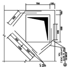
FOUNDATION REINFORCEMENT PLAN SEE 1200
