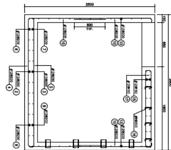
FOUNDATION REINFORCEMENT PLAN SEE 1200
