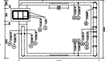
FOUNDATION REINFORCEMENT PLAN SEE 1200
