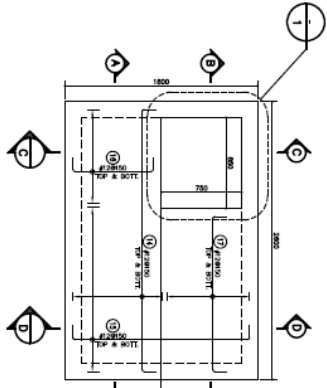
FOUNDATION REINFORCEMENT PLAN SEE 1200
