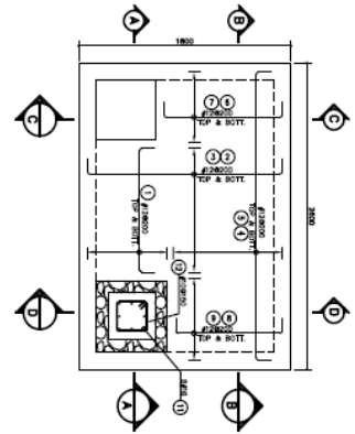
FOUNDATION REINFORCEMENT PLAN SEE 1200
