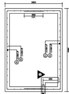
FOUNDATION REINFORCEMENT PLAN SEE 1200
