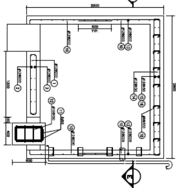
FOUNDATION REINFORCEMENT PLAN SEE 1200
