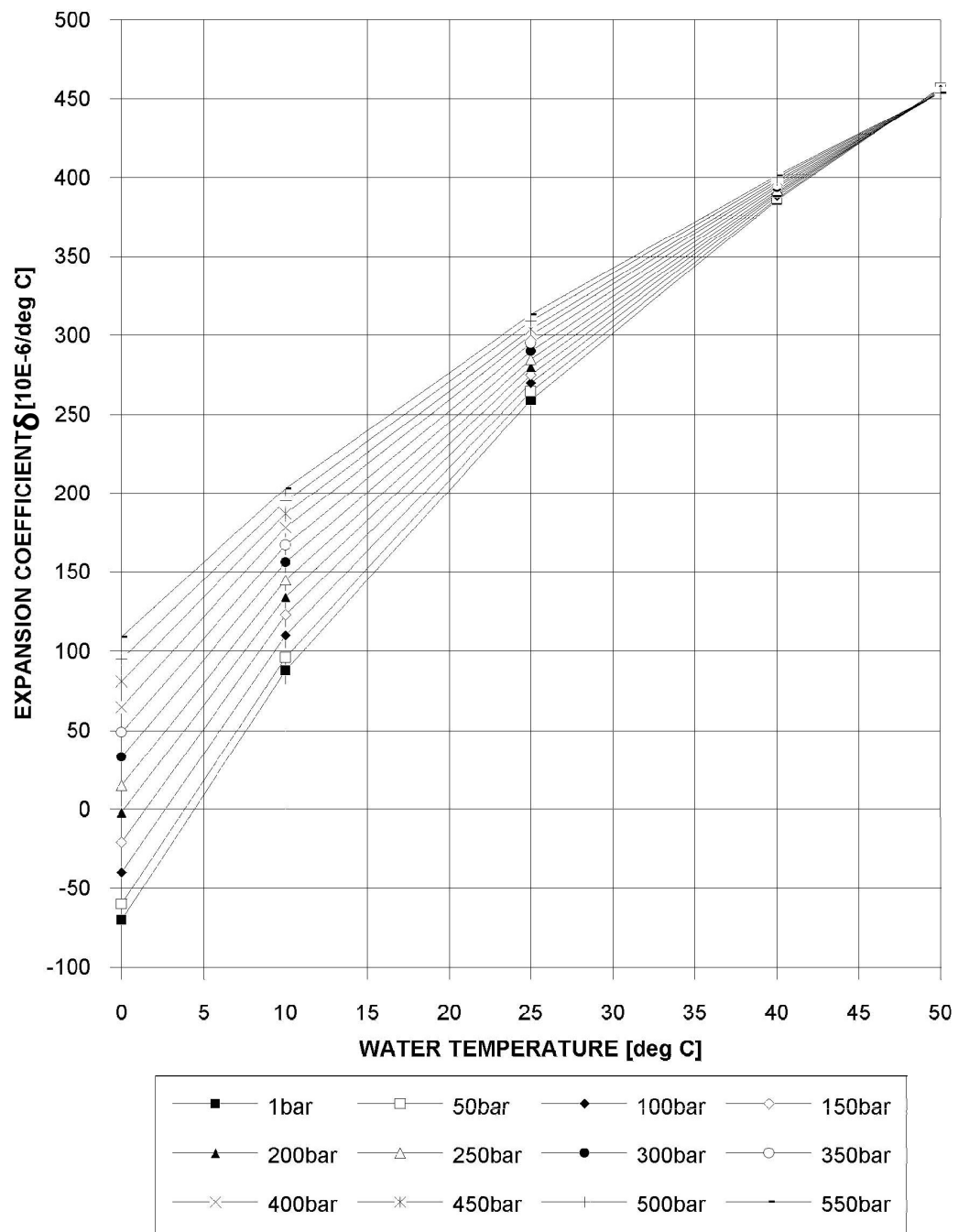
FIGURE 3 VOLUMETRIC EXPANSION COEFFICIENT OF FRESH WATER
