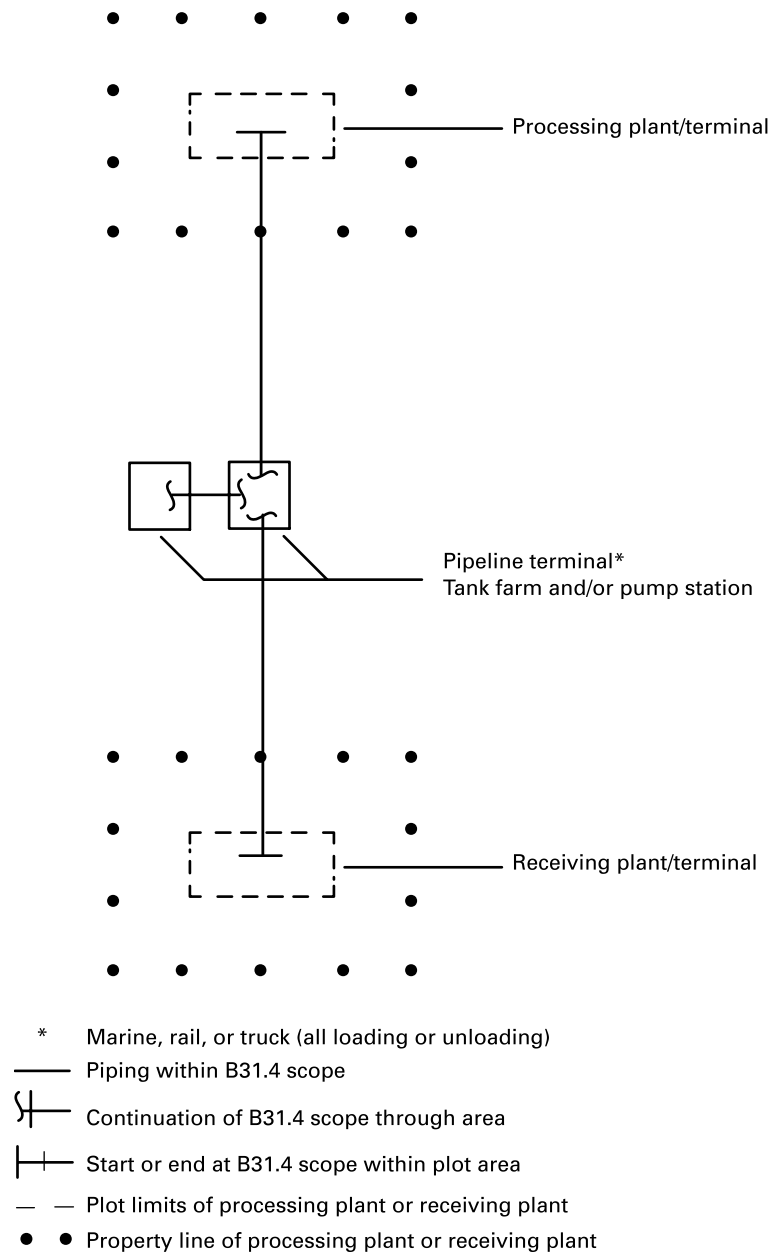
Figure 400.1.1-3 Diagram Showing Scope of ASME B31.4 for Slurry Pipeline Systems
