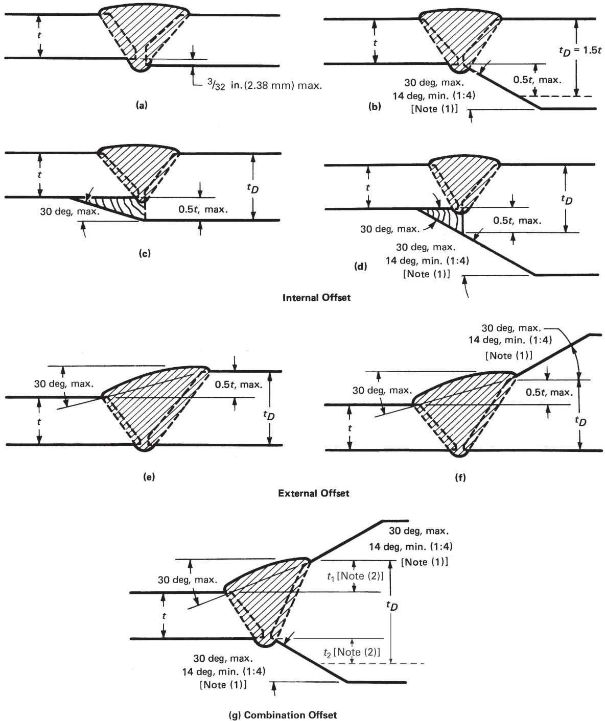
Figure I-5 Acceptable Design for Unequal Wall Thickness
