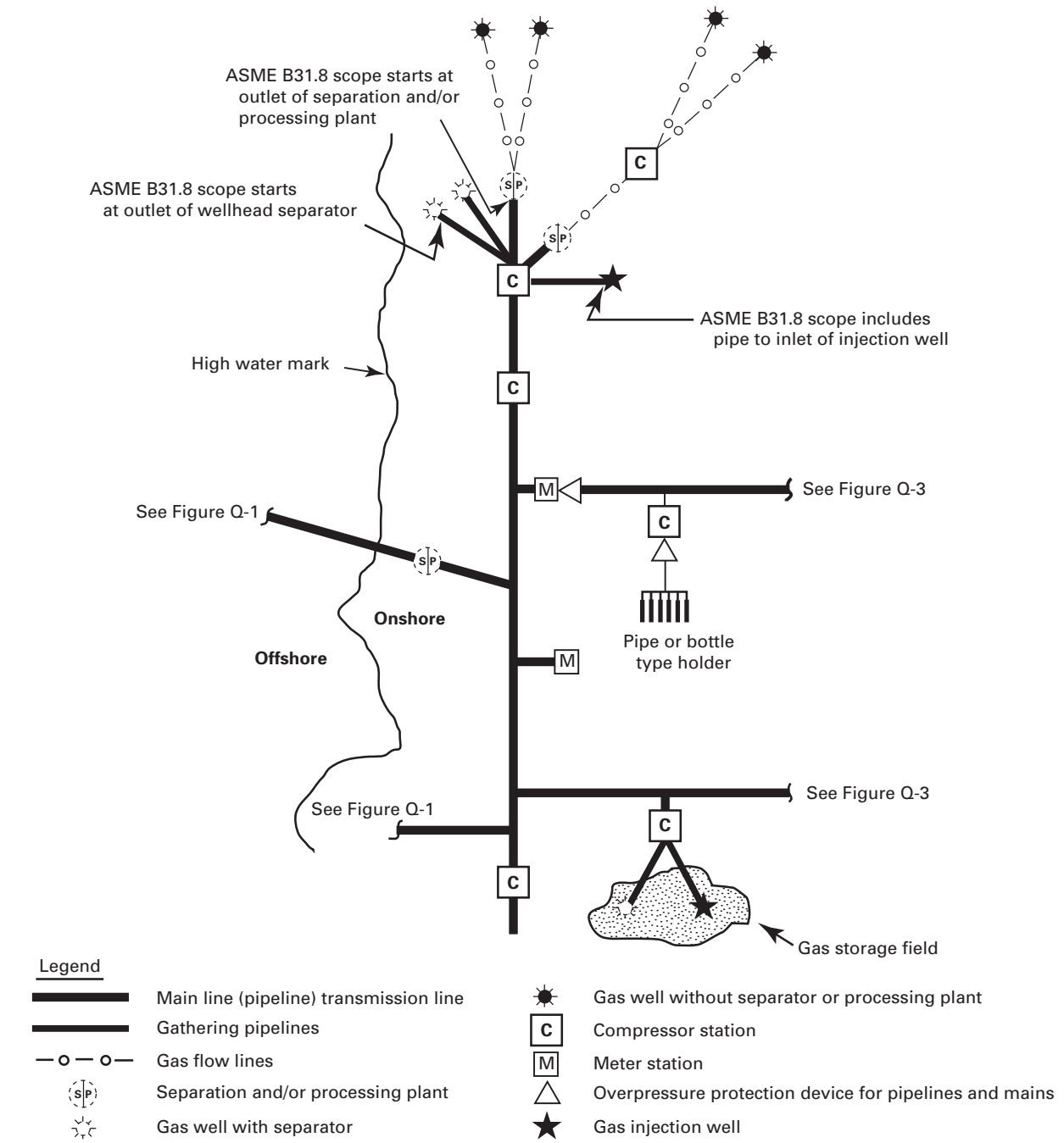
Figure Q-2 Scope of ASME B31.8 Transmission Piping Onshore
