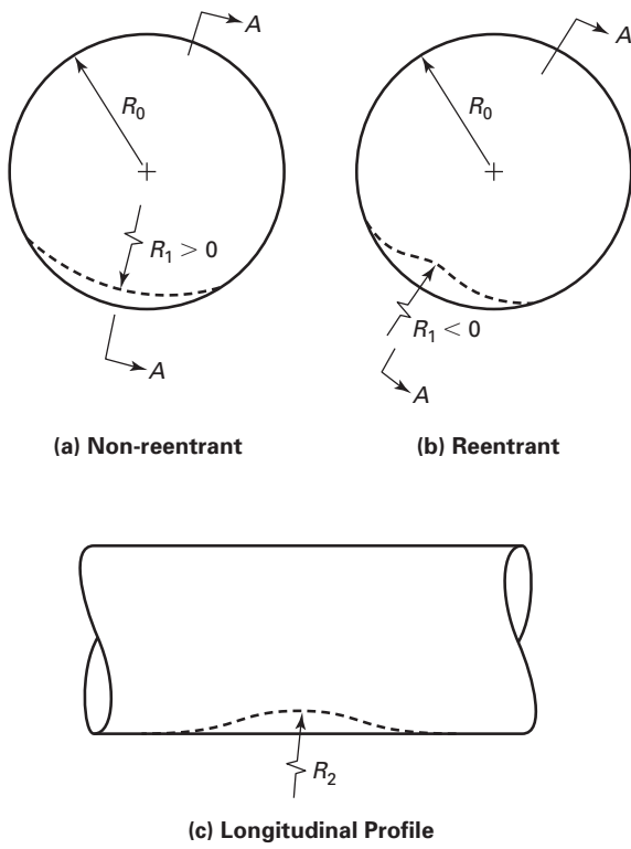
(20) Figure R-1 Method for Estimating Strain in Dents
