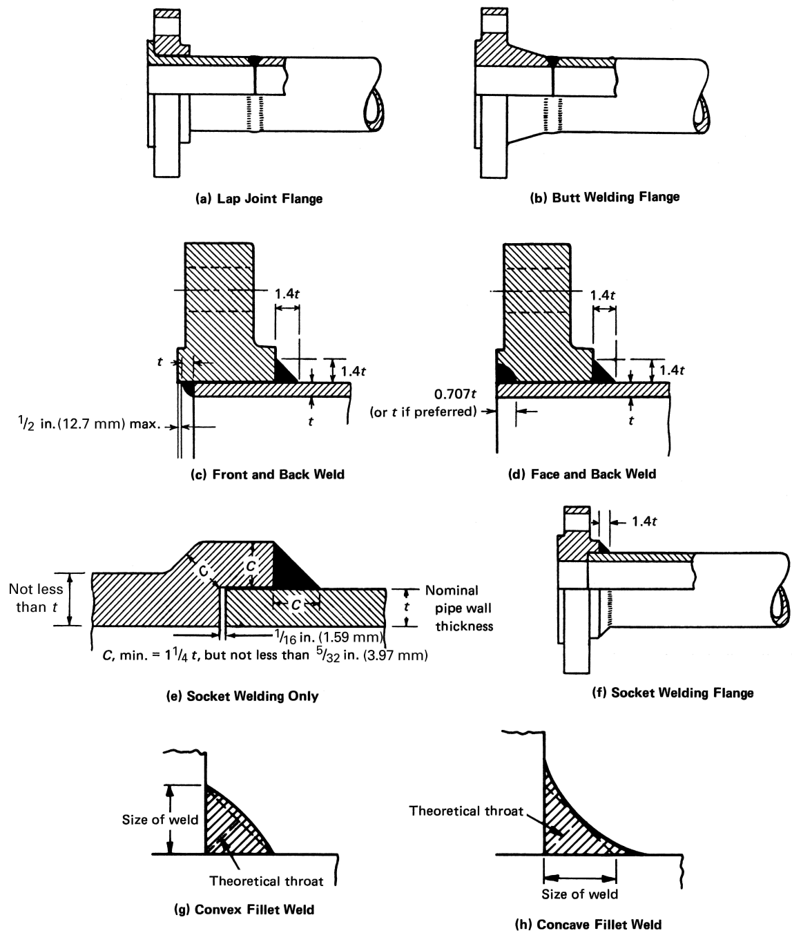
Figure I-6 Recommended Attachment Details of Flanges
