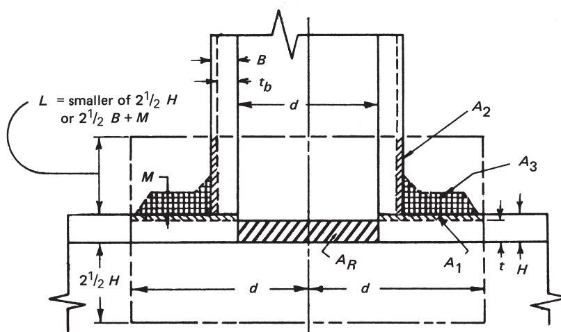
Figure F-5 Rules for Reinforcement of Welded Branch Connections
